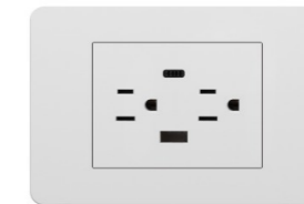
C1M6UC3 Duplex 3P socket with USB (A+C)
