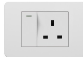
C111YS2/3 C112YS2/3 1 gang 1 way switch with 13A socket (2/3) 1 gang 2 way switch with 13A socket (2/3)
