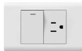
A1011M33/12M33 1 gang 1 way switch with 3P socket (3/3) 1 gang 2 way switch with 3P socket (3/3)
