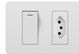
C111BX2/12BX2 1 gang 1 way switch with 3P socket (1/3) 1 gang 2 way switch with 3P socket (1/3)
