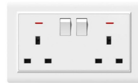
A10408 13A 2 gang SP switched socket, neon
