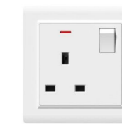
A10405 13A 1 gang switched socket A10409 13A 1 gang DP switched socket
