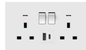
R10488C 13A 2 gang SP switched socket, 1 USB+1 type C, neon
