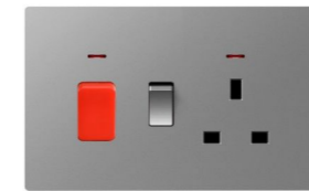
K331 45A DP switch with neon +13A switched socket with neon
