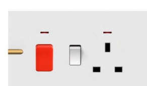
R11331 45A DP switch with neon +13A switched socket with neon
