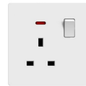
CN80411 13A 1 gang DP switched socket, neon
