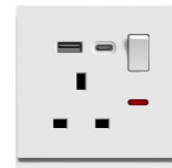
DN71491C 13A 1 gang DP switched socket, 1 USB + 1 type C, neon
