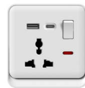
DN72587C 13A 1 gang switched MF socket, neon 1 USB + 1 type C
