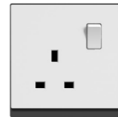
DN81405 13A 1 gang SP switched socket DN81409 13A 1 gang DP switched socket
