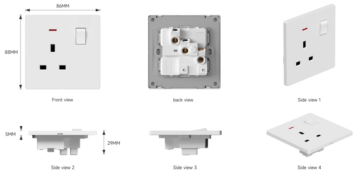
Metal supporting frame structure six views (socket)
